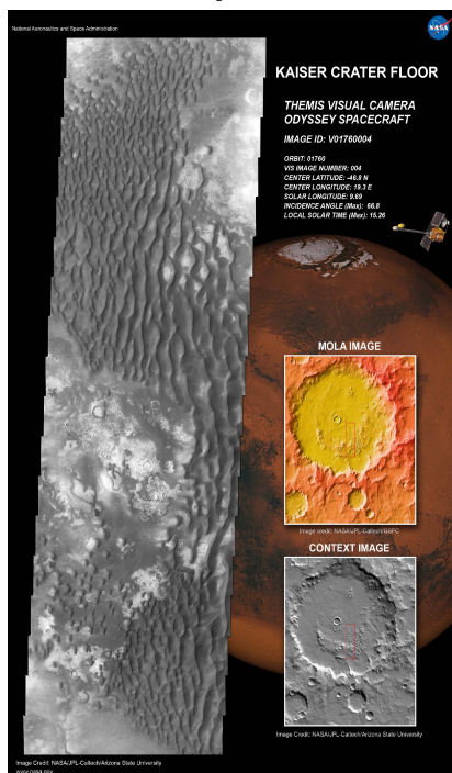
SAMPLE THEMIS IMAGE AND CONTEXT IMAGE
