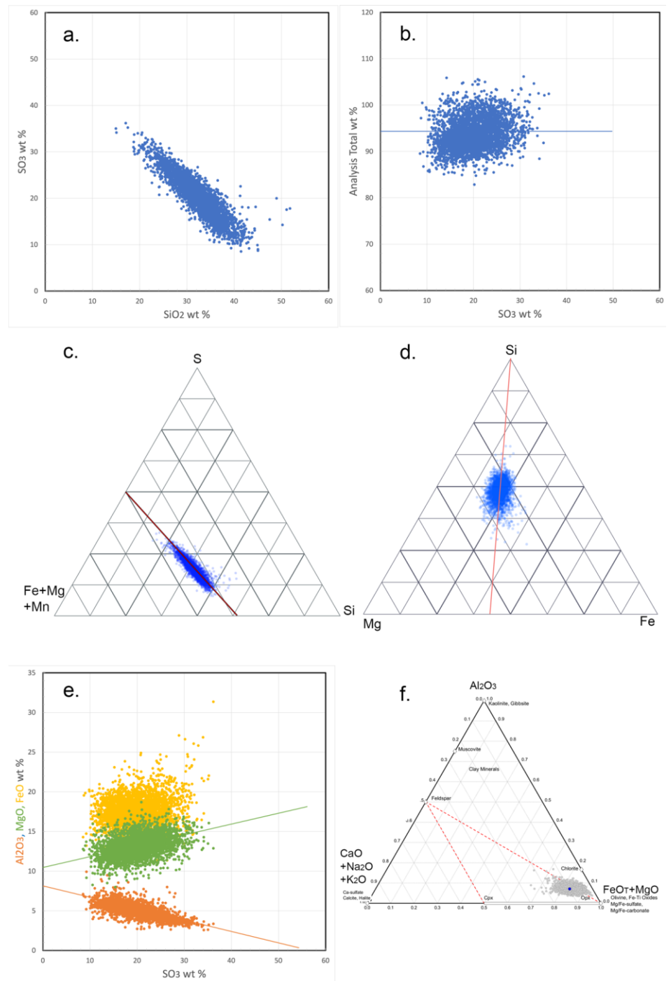
Figure 13 | Element abundance relations, PIXL scan Sol 505. (a) \text{SO}_3 vs \text{SiO}_2 . (b) Analytical sum vs \text{SO}_3 . (c) Ternary of molar S, Si, and Fe+Mg+Mn. (d) Ternary of molar Si, Mg, and Fe. (e) Multi-element correlations with \text{SO}_3 (f) Ternary of molar \text{Al}_2\text{O}_3 - (\text{CaO}+\text{Na}_2\text{O}+\text{K}_2\text{O}) - (\text{FeO}_T+\text{MgO}) , with common primary igneous and secondary minerals plotted for reference. The red dashed triangular envelope denotes a field in which mixtures of the primary igneous minerals olivine, pyroxene, and feldspar would plot.
