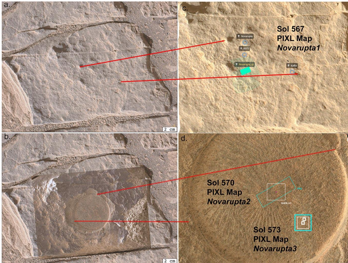
Figure 12 | PIXL raster scans on the Novarupta abrasion patch, sols 567, 570, and 0573. Green areas and outlines are the analysis footprints; white outlines are SHERLOC scans. (a) Novarupta area before abrasion (SI1-0566_0717192162_457ECM_N0290000SRLC04001_00000MJ01). (b) Novarupta area after abrasion (SI1-0566_07171381130_226ECM_N0290000SRLC02501_00000MJ01). (c) Location of the PIXL natural surface scan. Novarupta1 was a 5x7 mm map. (d) Locations of PIXL scans on abrasion patch, which is ~5 cm diameter. The 570 area was a 12.5x4 mm map; the 573 scan was an incomplete 7x7 mm grid.
