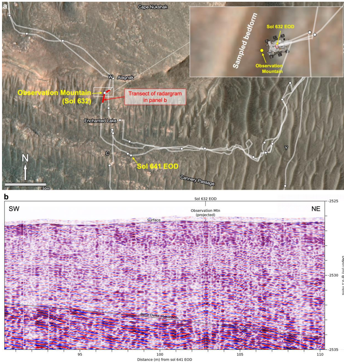
Figure 29. Geologic context and RIMFAX-derived subsurface stratigraphy of the delta front south of Cape Nukshak . (a) Location of the Observation Mountain megaripple. The inset shows detail of the sample location. The red line indicates the portions of the traverses on sols 632 and 641 during which RIMFAX radargrams were collected. (b) Radargram of the traverses shown by the red line in panel (a), leading to and away from the Observation Mountain megaripple.
