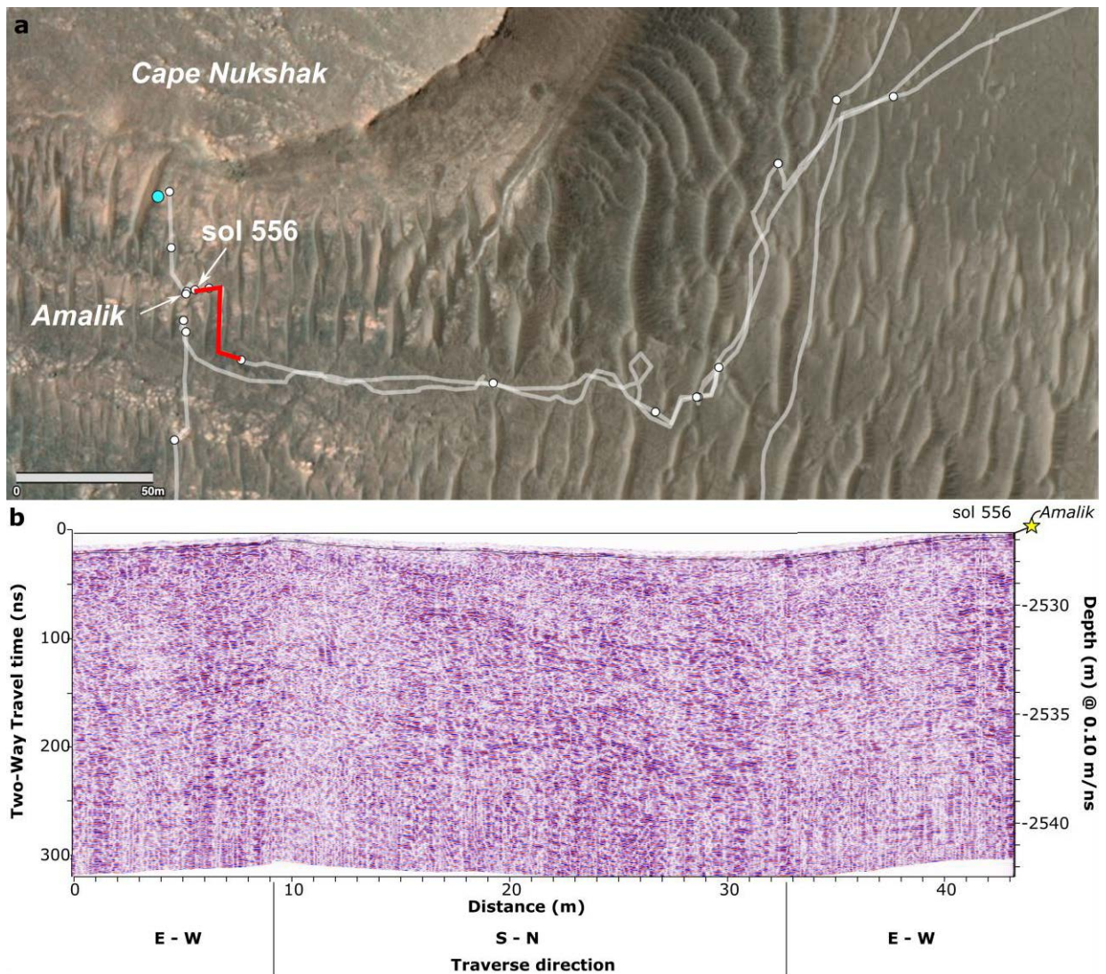
Figure 24 | Geological context and RIMFAX-derived subsurface stratigraphy of the delta front south of Cape Nukshak . (a) Location of the Amalik outcrop, from which the samples Shuyak and Mageik were collected, within the delta front. The red line indicates the traverse on sol 556 during which RIMFAX radargrams were collected. (b) Radargram of the three-leg traverse acquired on sol 556 ending near the Amalik outcrop (yellow star). The radargram shows strata with largely horizontal geometries above the Séítah Fm.
