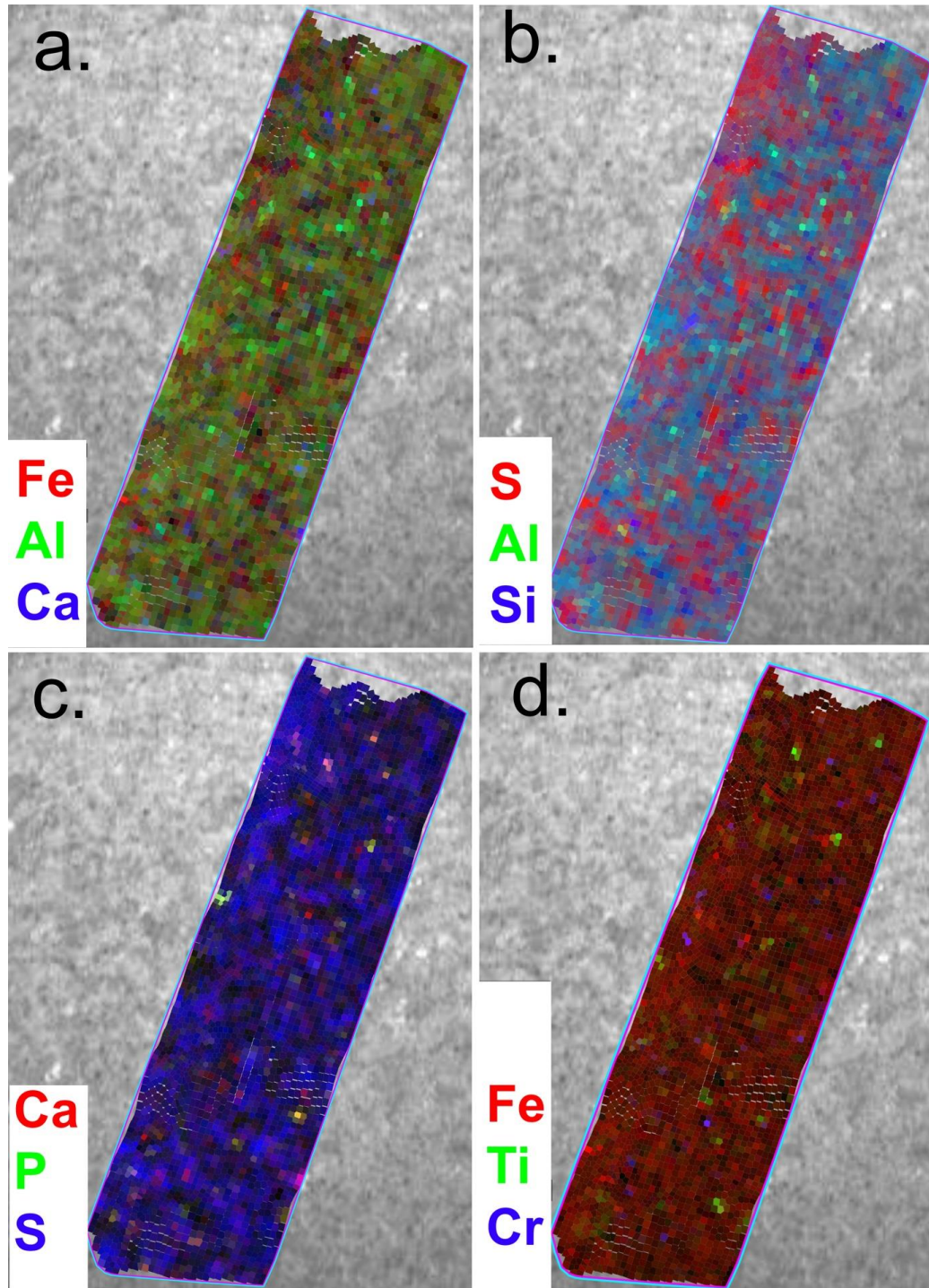
Figure 14 | PIXL multi-element maps for the Berry Hollow scan on Sol 505. (a) Red= \text{FeO}_T (10.8 to 30.4%), Green= \text{Al}_2\text{O}_3 (2.6 to 9.6%), Blue= \text{CaO} (0.4 to 7.5%). The few green spots represent an Al-rich phase, likely the purest areas of the silicate mineral (Figure 13e). (b) Red= \text{SO}_3 (8.5 to 34.9%), Green= \text{Al}_2\text{O}_3 (2.6 to 9.6%), Blue= \text{SiO}_2 (15.0 to 51.0%). The analysis spots in red-purple-blue represent mixtures of the sulfate and silicate phases (Figure 13c). (c) Red= \text{CaO} (0.4 to 7.5%), green= \text{P}_2\text{O}_5 (0.0 to 8.0%), blue= \text{SO}_3 (8.5 to 34.9%). Yellow and green analysis spots are rich in Ca & P and are inferred to be calcium phosphates. The purple spots are rich in Ca sulfate. (d) Red= \text{FeO}_T (10.8 to 30.4%), green= \text{TiO}_2 (0.2 to 7.6%), blue= \text{Cr}_2\text{O}_3 (0.0 to 5.1%). Purple and green spots might represent chromium- and titanium-rich Fe oxides.
