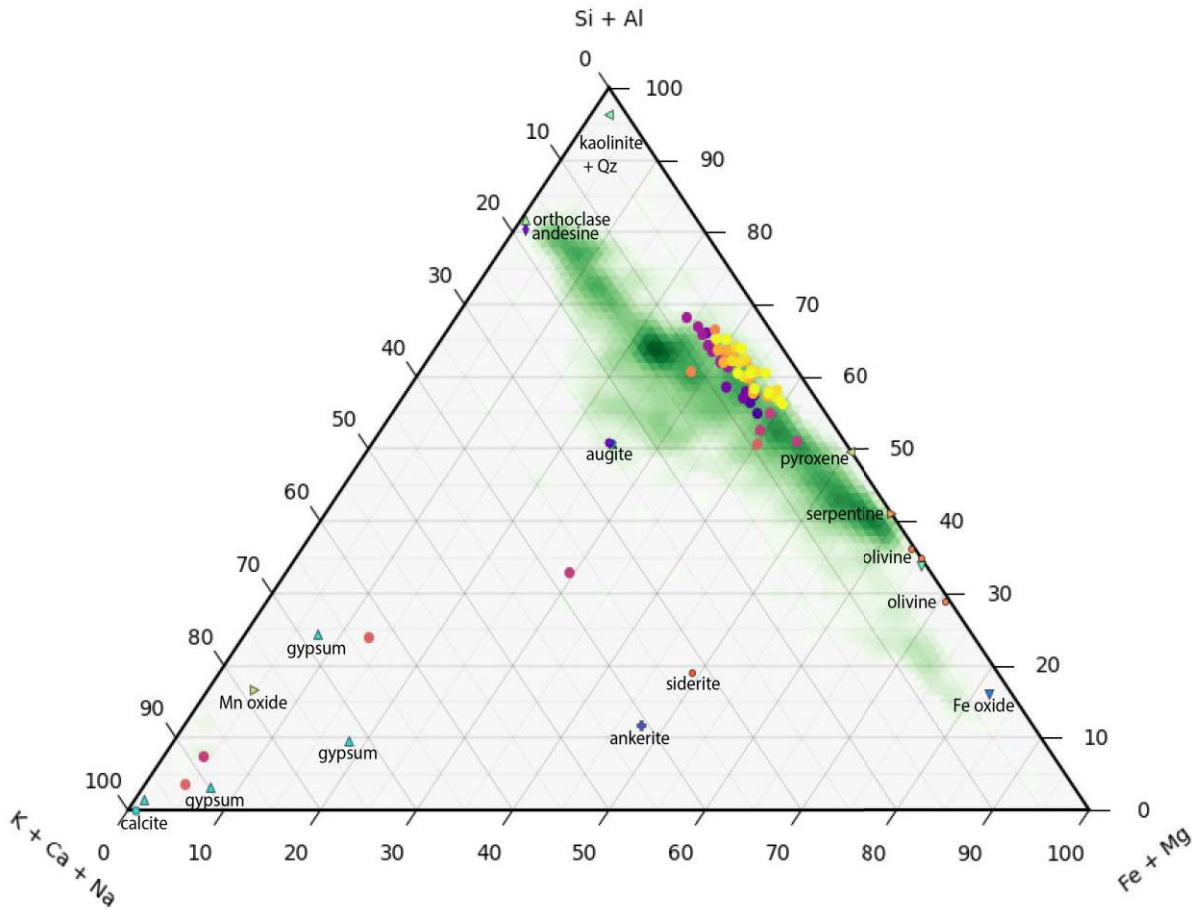
Figure 21 | Molar compositions of the points in the SCAM LIBS raster of Wildcat Ridge . Data are from Sols 507, 511, 515, 517, 520, 521, 522 and 531 compared to various minerals and on-board calibration standards. Blue and purple circles show points analyzed on the natural surface targets Bearwallow on Sol 511 and Hogback Mountain on Sols 520 and 531. Fuchsia and red circles show the composition of the points analyzed on target Mill Prong from Sols 517 and 521. This target contained a vein enriched in calcium; points analyzed in this vein cluster with gypsum in the left lower corner of the ternary diagram. Orange circles show points on the abraded patch Berry Hollow analyzed on Sols 507 and 515. Darker and lighter yellow circles show the composition of the tailings on the target Hazeltop on Sols 511 and 522. The legend presents a range of standards from igneous calibration targets (Ca-pyroxene, pyroxene, olivine) to other minerals (calcite, ankerite, siderite, serpentine, gypsum). The green cloud shows all data points acquired up to Sol 540.
