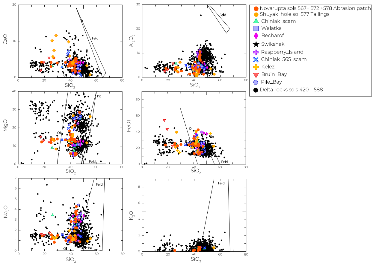
Figure 21 | SuperCam LIBS major element oxide (MOC) analyses of Amalick rocks. Solid solution fields for olivine, pyroxene, and feldspar compositions are included. Black spots show the delta rocks analyzed from Sols 420–588.
