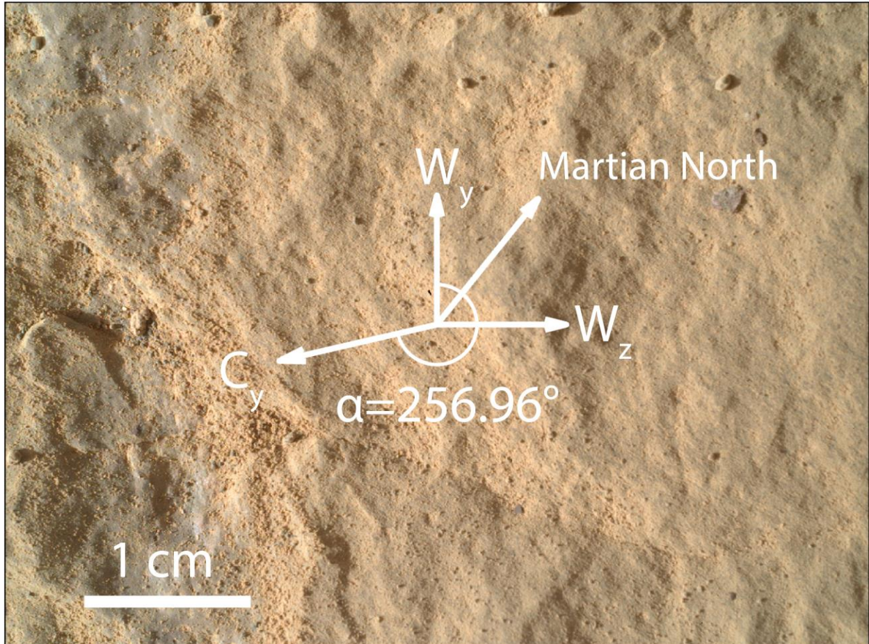
Figure 25 | 6.8-cm standoff WATSON image of Shuyak core target on sol 570. WATSON image SIF_0570_0717551784_765FDR_N0290000SRLC00750_0000LMJ01. Image scale is 31.6 \mu\text{m pixel}^{-1} . Orientation compass gives WATSON frame ( w_x , w_y , w_z ). Core roll is clockwise angle of core y-axis, c_y , from w_y , given by \alpha = 256.96^\circ . Projection of Martian geographic north onto WATSON image plane is noted.
