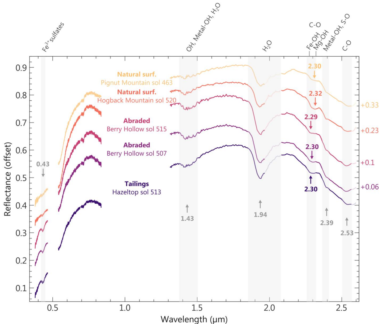
Figure 22 | Mean reflectance spectra of the SuperCam VISIR rasters on the Wildcat Ridge outcrop. Mean reflectance spectra of the SuperCam VISIR rasters on the Wildcat Ridge outcrop (abraded surface and tailings from coring activity). Lighter lines near 2 \mu\text{m} indicate the spectral range possibly affected by the CO 2 absorption features that could remain after the atmospheric correction. The UV region was smoothed using a Savitzky-Golay filter. Note that owing to temperature sensitivities in the IRS instrument, the calibration is still uncertain for wavelength longer than \sim 2.55 \mu\text{m} . The absorption centers are indicated with arrows and their positions point towards the presence of hydrated minerals: sulfates with the absorption around 2.39 \mu\text{m} , Fe/Mg-phyllsilicates with the absorption at 2.23 and around 2.3 \mu\text{m} and/or carbonates.
