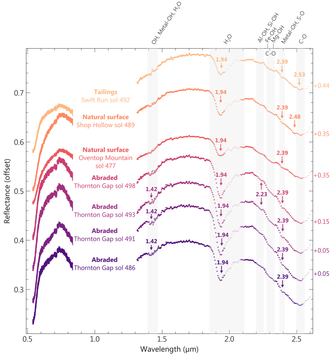
Figure 23 | Mean reflectance spectra of the SuperCam VISIR rasters on the Skinner Ridge outcrop. Natural surface (orange and red), abraded surface (purple to red) and tailings from abrading activity (yellow). Lighter points near 2 \mu\text{m} indicate the spectral range possibly affected by the \text{CO}_2 absorption features after the atmospheric correction. Note that owing to temperature sensitivities in the IRS instrument, the calibration is still uncertain for wavelength longer than \sim 2.55 \mu\text{m} . Arrows indicate the absorption bands arising from the presence of hydrated minerals. Arrows in the 2.1-2.5 \mu\text{m} range point towards weak absorptions indicating small amounts of Fe/Mg-clay minerals, possible carbonates, and hydrated silica or Al-clay minerals.
