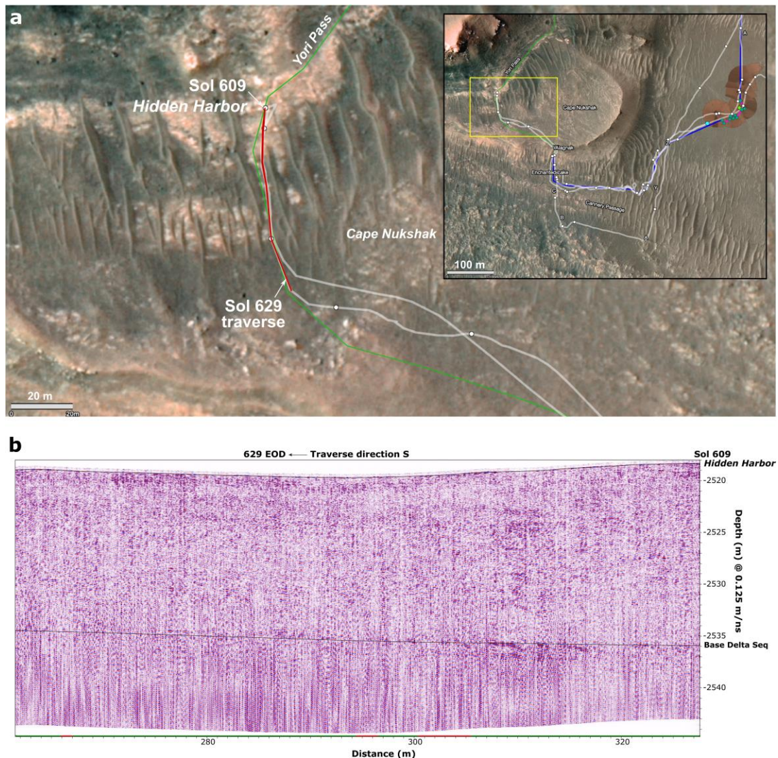
Figure 23 | Geological context and RIXFAX-derived subsurface stratigraphy of the delta front on the western side of Cape Nukshak. (a) Location of the Hidden Harbor outcrop, from which the samples Kukaklek was collected, within the delta front. The inset shows the broader context of the sample location. The red line indicates the beginning of the traverse on Sol 629 during which RIMFAX radargrams were collected. (b) Radargram of the multileg traverse acquired on Sol 629 beginning near the Hidden Harbor outcrop. The radargram shows strata with largely horizontal geometries above the Séítah Fm.
