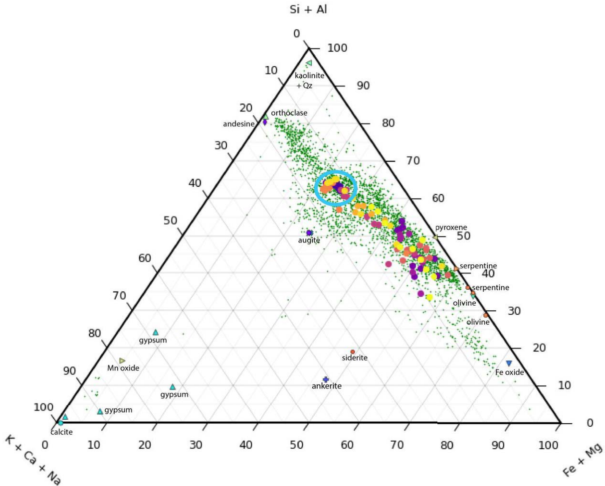
Figure 22 | Molar compositions of the points in the LIBS rasters of Amalik from Sols 558, 561, 563, 565-567, 572, 577 and 578 compared to various minerals and on-board calibration standards. Analyzed points are shown by the yellow, orange, red, fuchsia, dark blue and purple circles. Purple and fuchsia circles show points analyzed on the abraded patch Novarupta from sols 572 and 578. Dark blue and dark and bright red circles, respectively, show the natural surfaces of Novarupta target from Sol 567 and Chiniak target from Sol 558 and 565, respectively. Dark and light orange circles, respectively, show the natural surfaces of Swikshak target from Sol 563 and Walatka target from Sol 561, respectively. Lemon yellow circles show the natural target Raspberry_Island analyzed on Sol 565. Marigold circles show the composition of the tailings from Shuyak drillhole analyzed on Sol 577. Turquoise circle surrounds the points analyzed on the shiny surface coatings. The legend presents a range of standards from igneous calibration targets (Ca-pyroxene, pyroxene, olivine) to other minerals (calcite, ankerite, siderite, serpentine, gypsum). The green cloud shows all data points acquired up to Sol 588.
