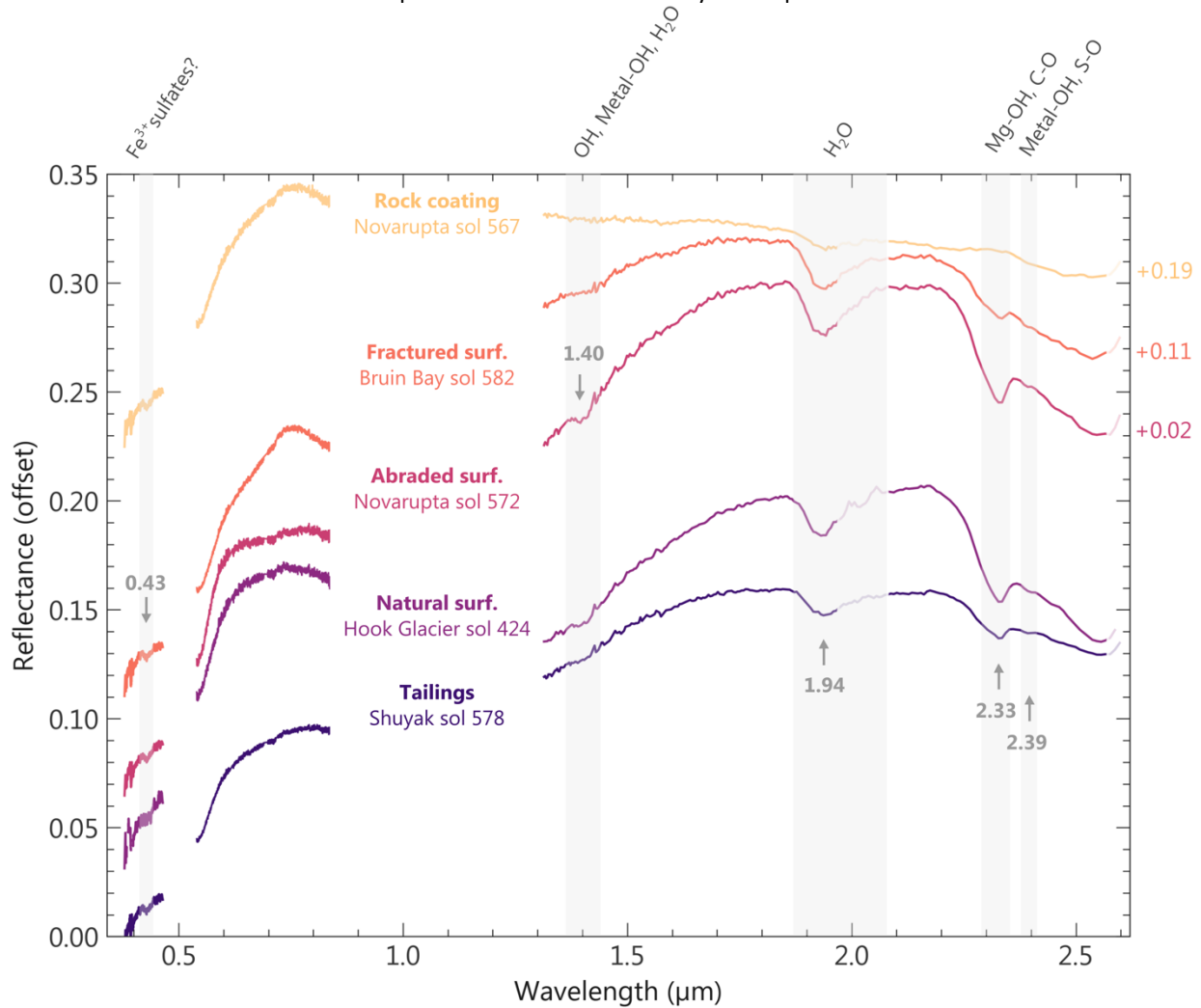
Figure 23 | Mean reflectance spectra of the SuperCam VISIR rasters at Amalik. These spectra show the natural surface of the Hook Glacier target observed on Sol 424, the abraded surface of Novarupta target from Sol 572 and tailings created by the coring of Shuyak . Also shown is the spectrum of the coating around the abraded surface at Novarupta analyzed on Sol 567. Lighter spectrum lines near 2 \mu\text{m} indicate the spectral range possibly affected by the \text{CO}_2 absorption features that could remain after the atmospheric correction. The UV region was smoothed using a savgol filter. Note that owing to temperature sensitivities in the IRS instrument, the calibration is still uncertain for wavelength longer than \sim 2.55 \mu\text{m} . The absorption centers are indicated with arrows and their positions at 1.94 and 2.33 \mu\text{m} point towards the presence of hydrated magnesium phyllosilicates, likely serpentine. Other arrows indicate additional absorption centers attributed to hydrated phases.
