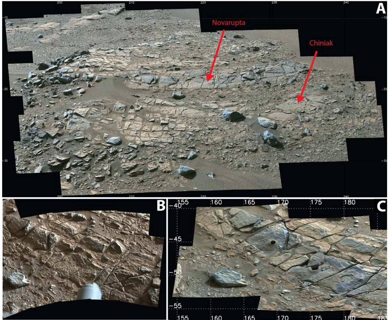
Figure 5 | Mastcam-Z context images for the Amalik outcrop. (a) The Amalik workspace; Novarupta and Chiniak targets are indicated. Sol 557, zcam08578, Z110 enhanced color. (b) The unmodified workspace ZCAM mosaic. Sol 565, zcam07101, Z110 enhanced color. (c) The workspace after abrasion and sampling activities, showing the fracturing that occurred after Shuyak was cored (center) and the regolith that settled during abrasion of the Novarupta abrasion (right) and sampling of Mageik (left). Sol 582, zcam08595, Z63 enhanced color.
