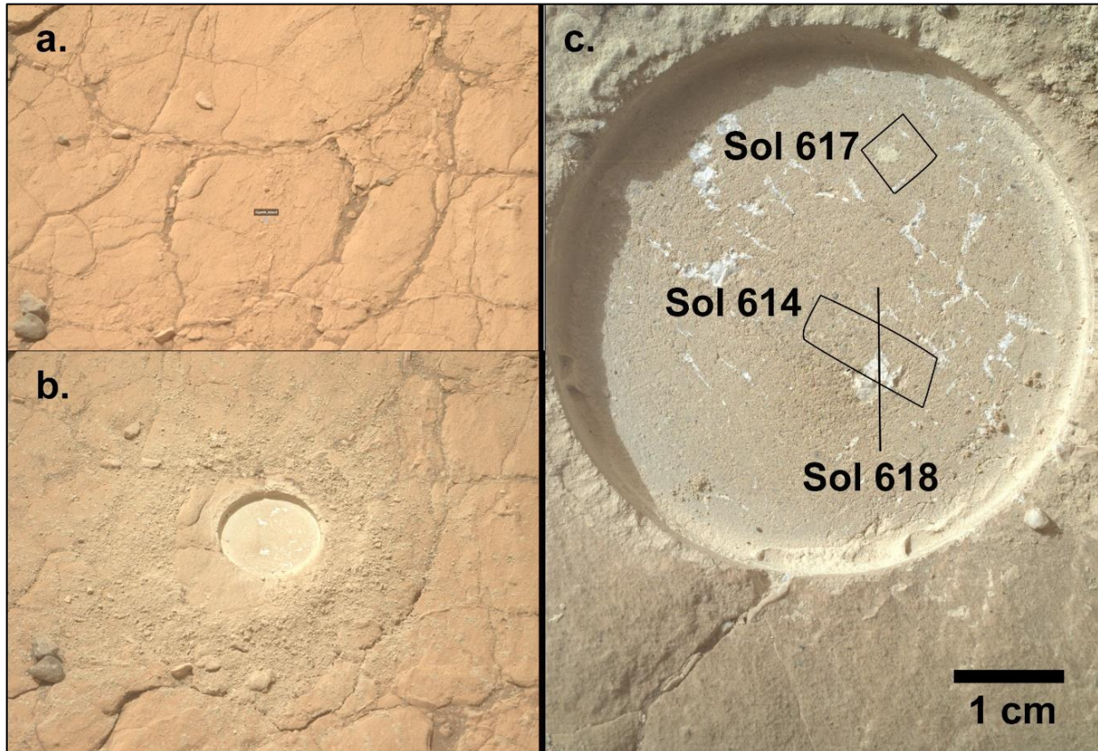
Figure 12 | PIXL raster scans on the Uganik Island abrasion, sols 614, 617, and 618. (a) Pre-abrasion (ZCAM image ZRF_0612_0721272628_348FDR_N0301172ZCAM03480_1100LMJ01). (b) Post-abrasion, abrasion is 5 cm diameter (ZCAM ZLF_0613_0721362736_818FDR_N0301172ZCAM03483_1100LMJ01). (c) Detail of abrasion, rotated slightly from part (b). PIXL scan locations & Sol annotated onto WATSON image SIF_0612_0721282138_906FDR_N0301172SRLC00746_0000LMJ01.
