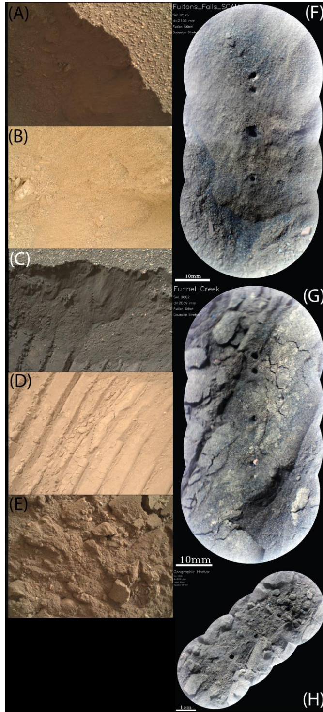
Figure 12 | Wheel-scuff documentation images and areas of analysis. WATSON image at (A) ~25 cm standoff and (B) ~9 cm standoff images of the surface-scarp interface. (C) ZCAM image of the surface-scarp interface and (D) of the wheel track. (E) Excavated regolith imaged with WATSON at ~ 7 cm standoff ( Topographers Peak ). Gaussian stretched RMI of (F) post LIBS analysis of Fultons Falls , (G) Funnel Creek and (H) Geographic Harbor .
